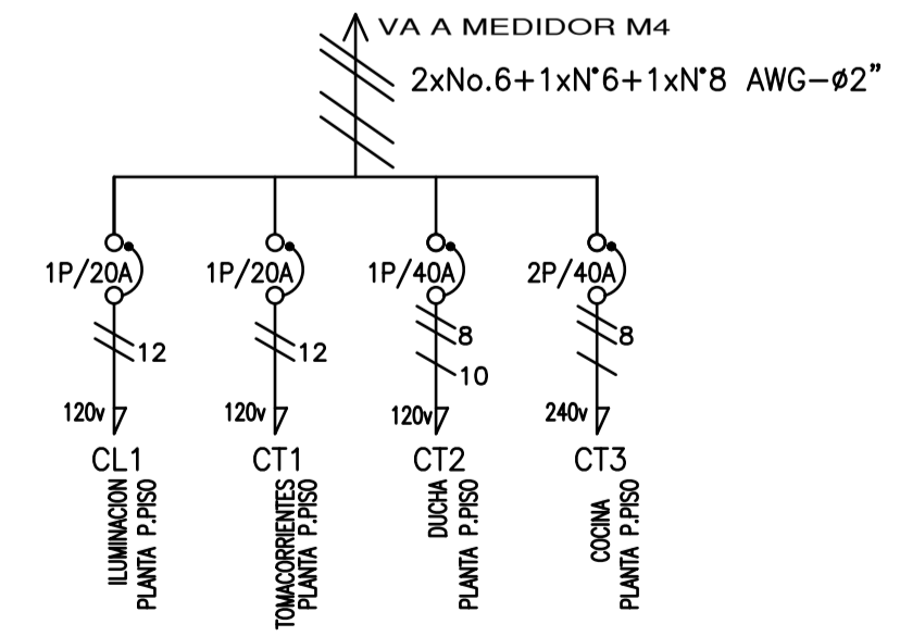
DIAGRAMA UNIFILAR TC3
