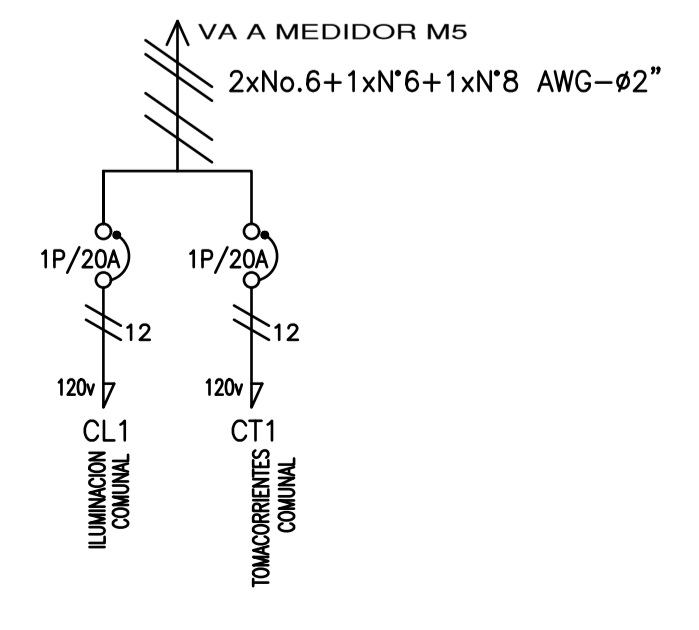
DIAGRAMA UNIFILAR TC3
