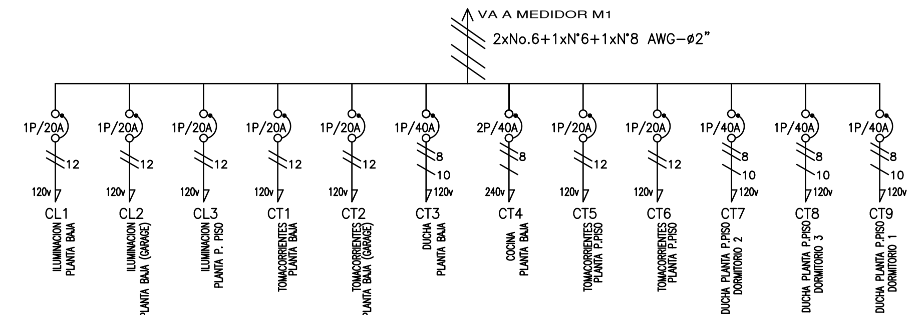
DIAGRAMA UNIFILAR TC1
