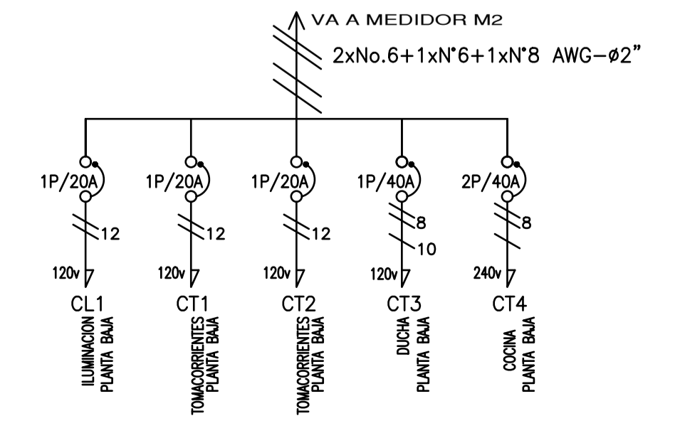
DIAGRAMA UNIFILAR TC2
