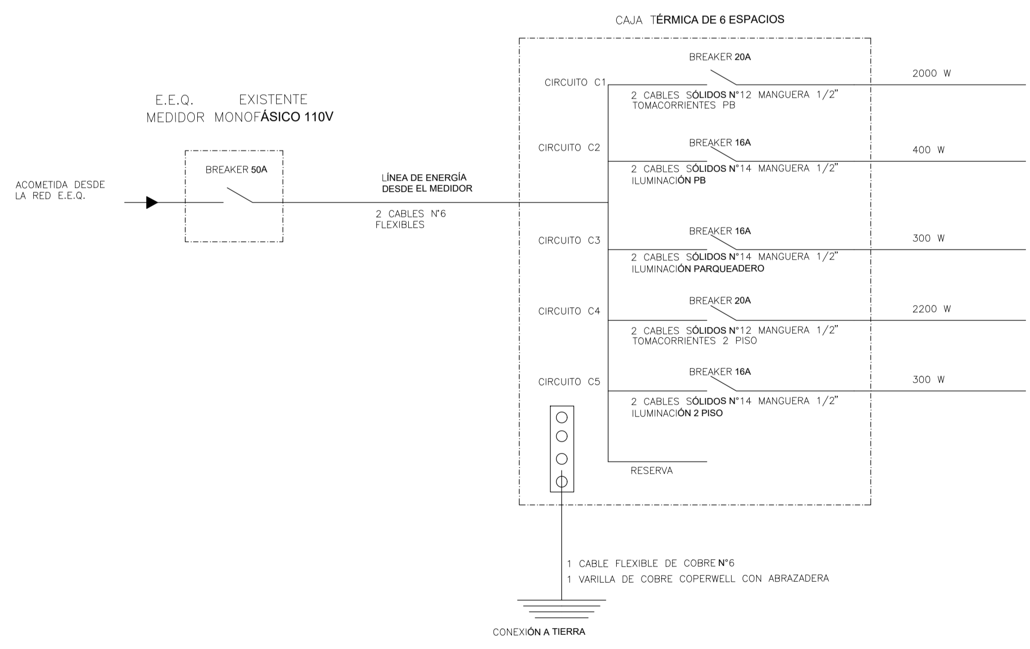
DIAGRAMA UNIFILAR
